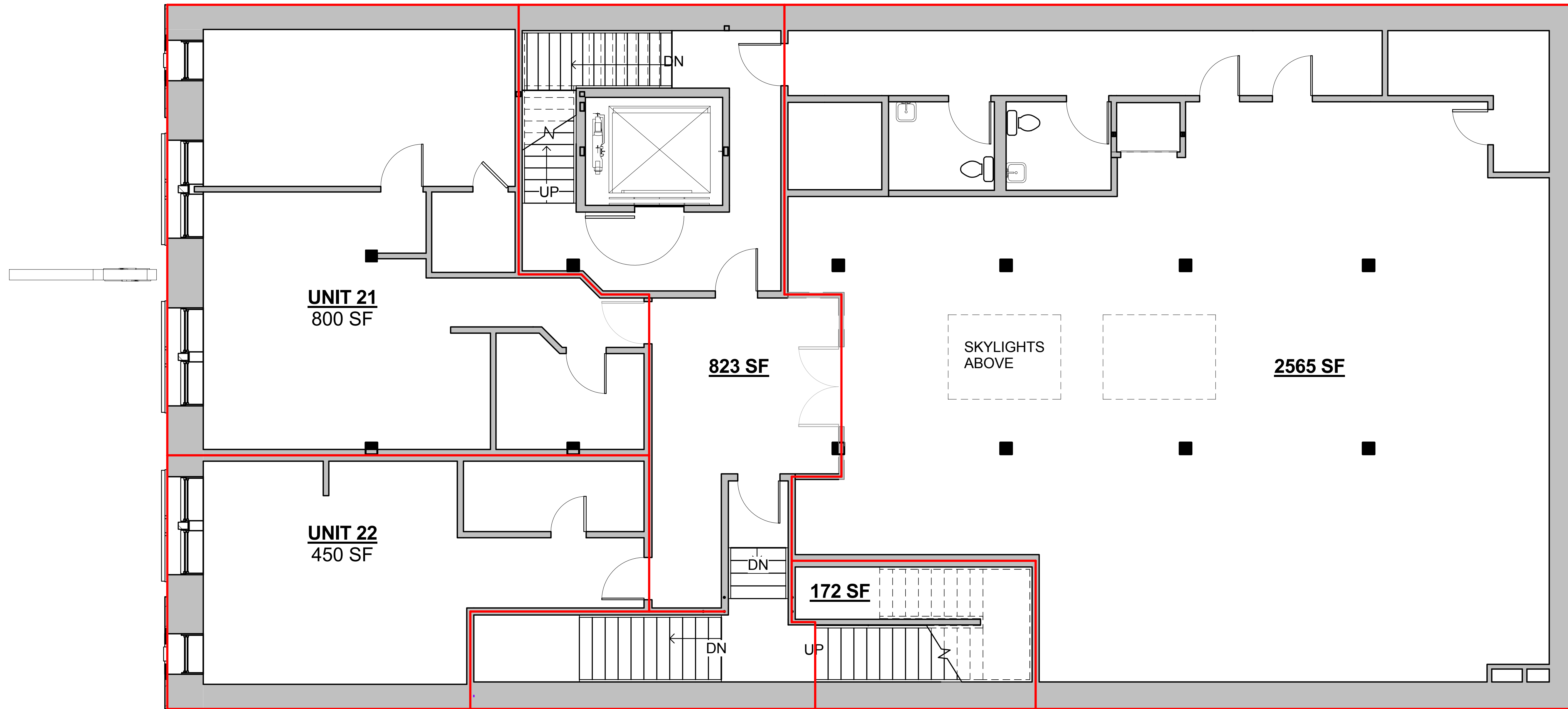
1 (M) 2ND AREA PLAN M2 SCALE: 1/8" = 1'-0"
